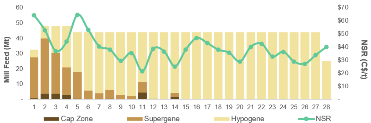
Figure 9. Process Plant Feed by Ore Type
